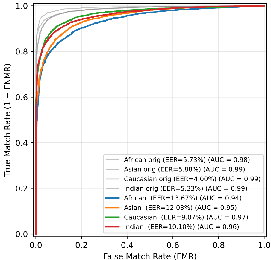
ROC — Contrast ( \alpha=0.2 )
