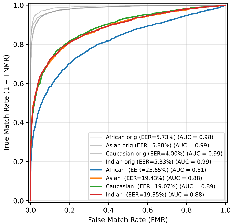
ROC — Contrast ( \alpha=4 )
