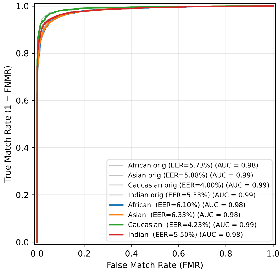
ROC — Gaussian Blur ( \sigma=0.8 )
