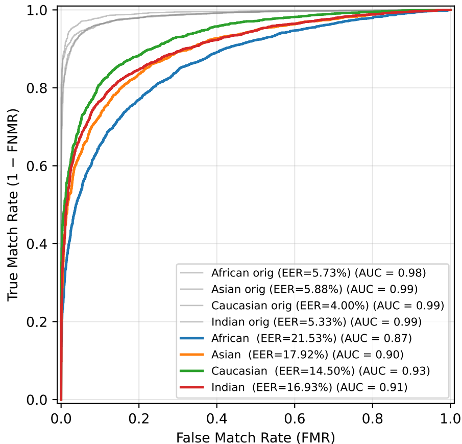
ROC — Gaussian Blur ( \sigma=2.6 )
