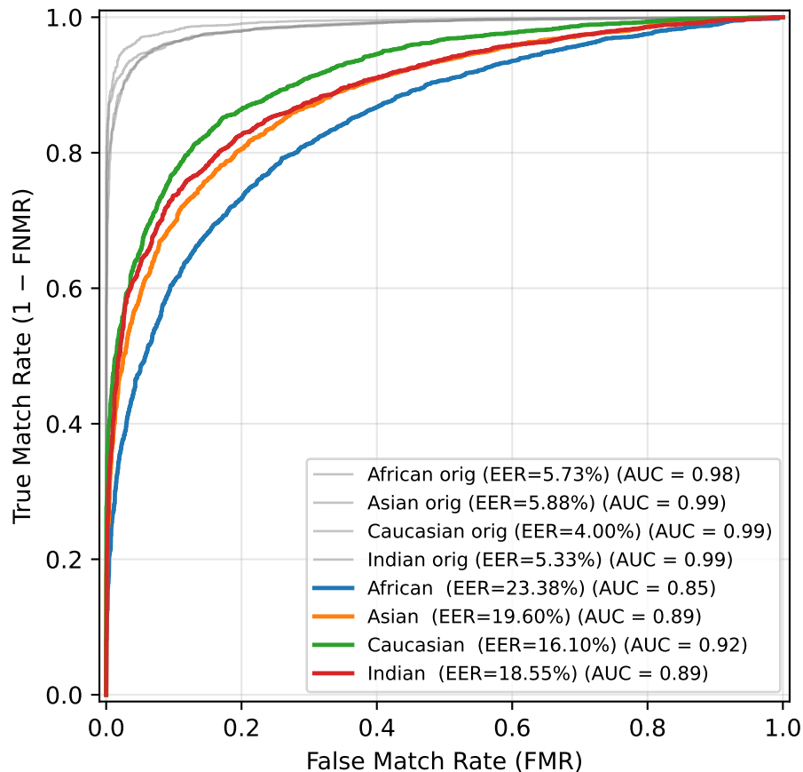
ROC — Gaussian Blur ( \sigma=2.8 )
