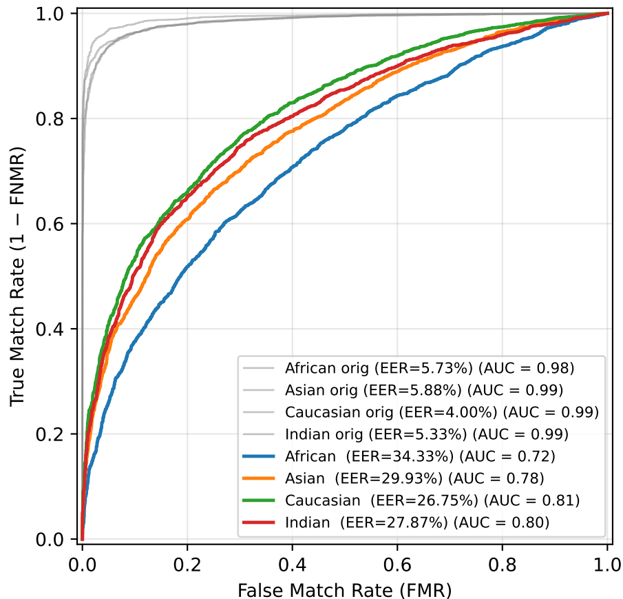
ROC — Gaussian Blur ( \sigma=4 )
