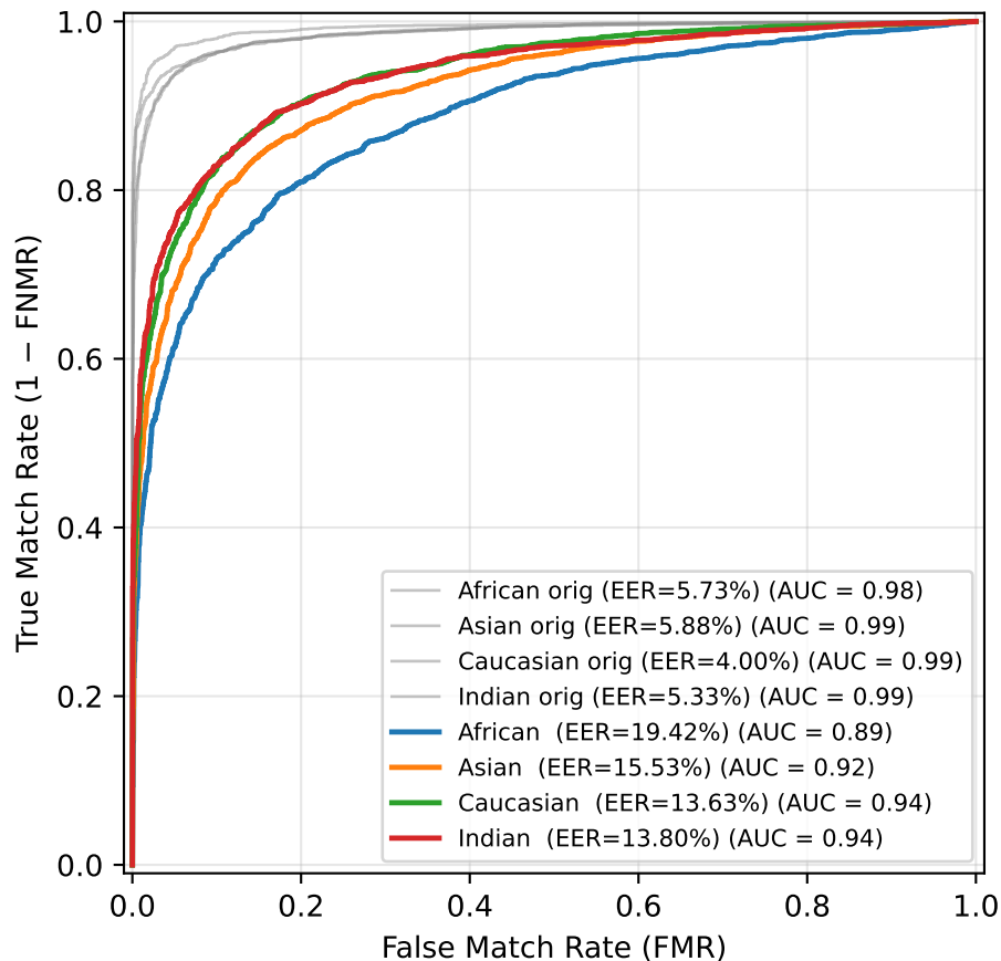
ROC — Gaussian Noise ( \sigma=20 )
