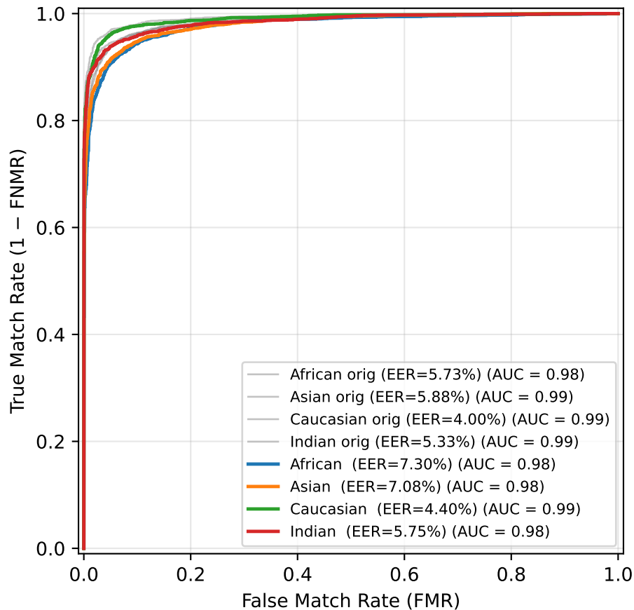
ROC — Gaussian Noise ( \sigma=4 )
