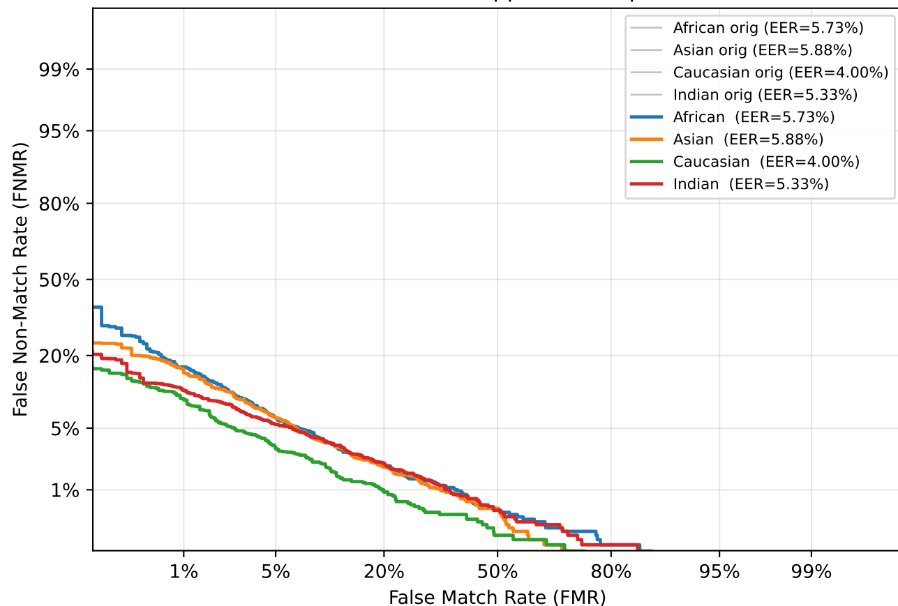
DET — Salt & Pepper Noise (p=0)
