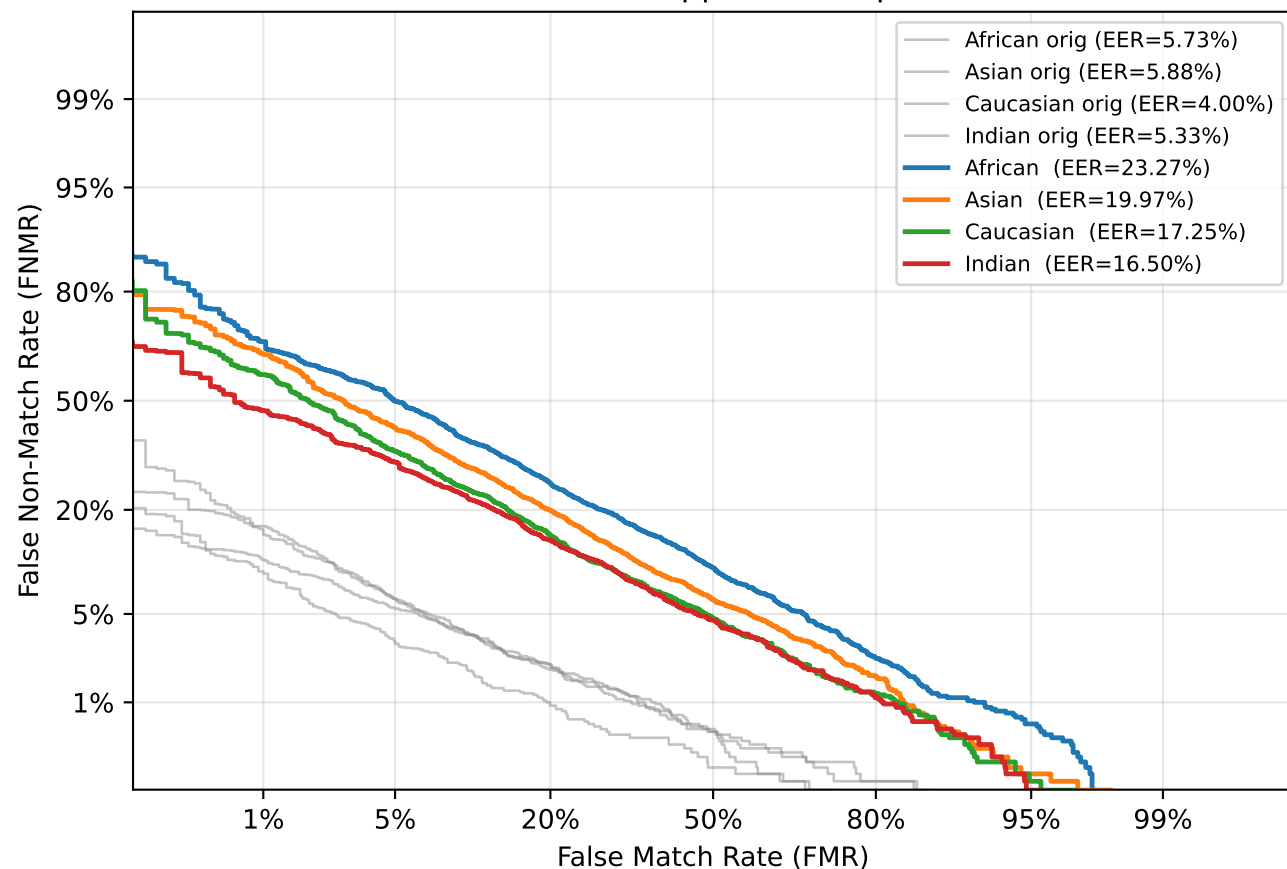
DET — Salt & Pepper Noise (p=0.06)
