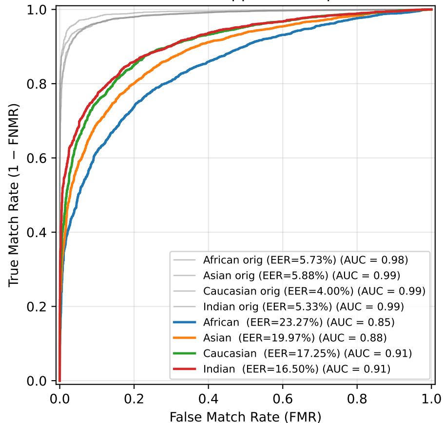
ROC — Salt & Pepper Noise (p=0.06)
