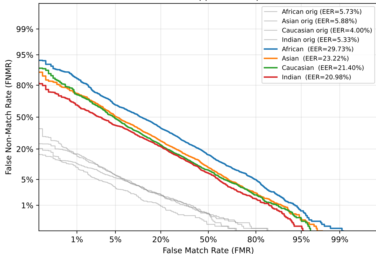
DET — Salt & Pepper Noise ( p=0.09 )
