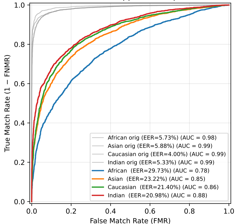
ROC — Salt & Pepper Noise ( p=0.09 )
