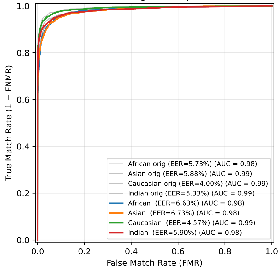
ROC — Brightness ( \beta=0.5 )
