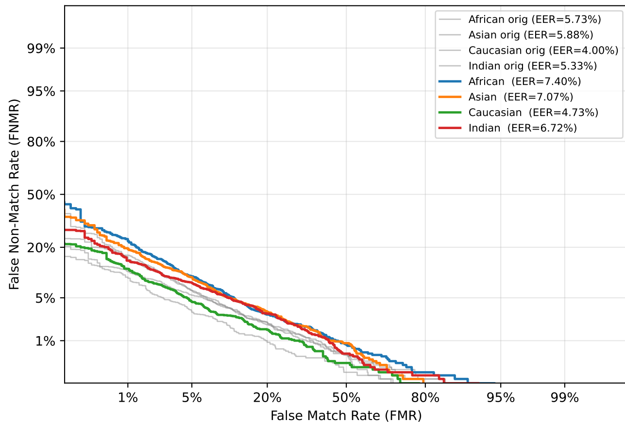
DET — Contrast ( \alpha=1.5 )
