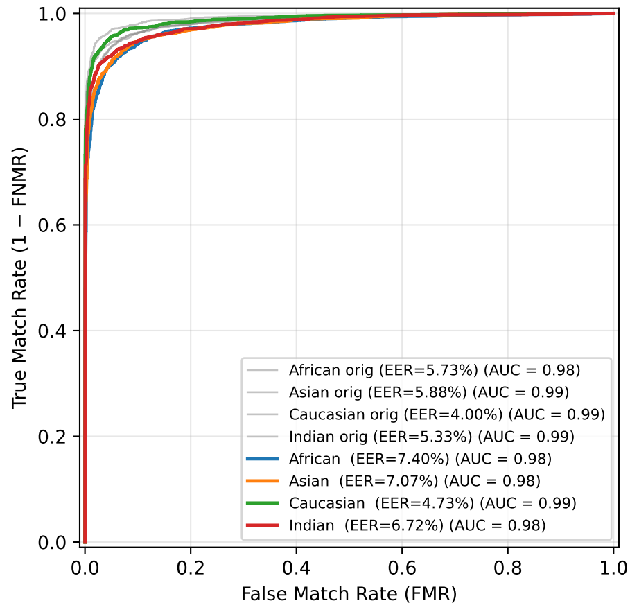
ROC — Contrast ( \alpha=1.5 )
