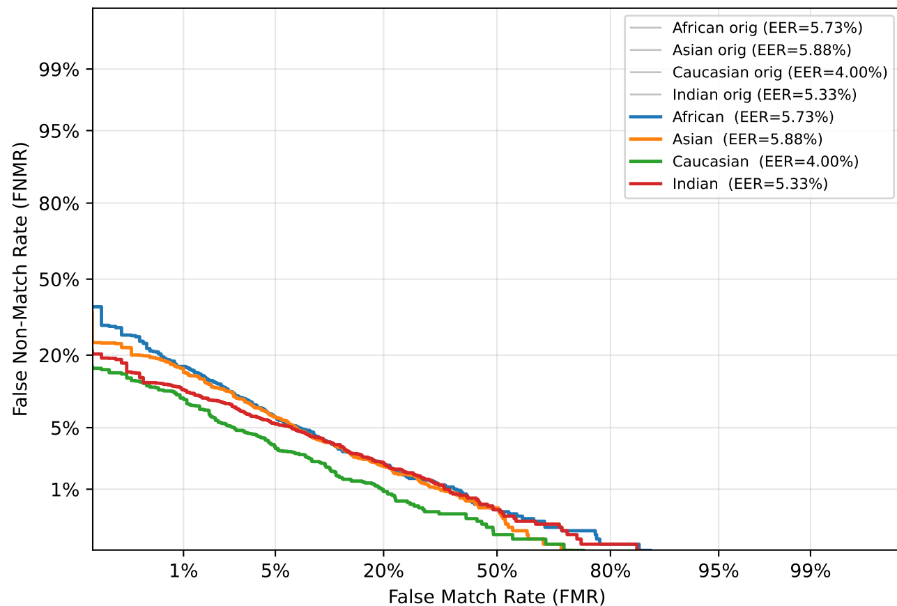
DET — Gaussian Blur ( \sigma=0.2 )
