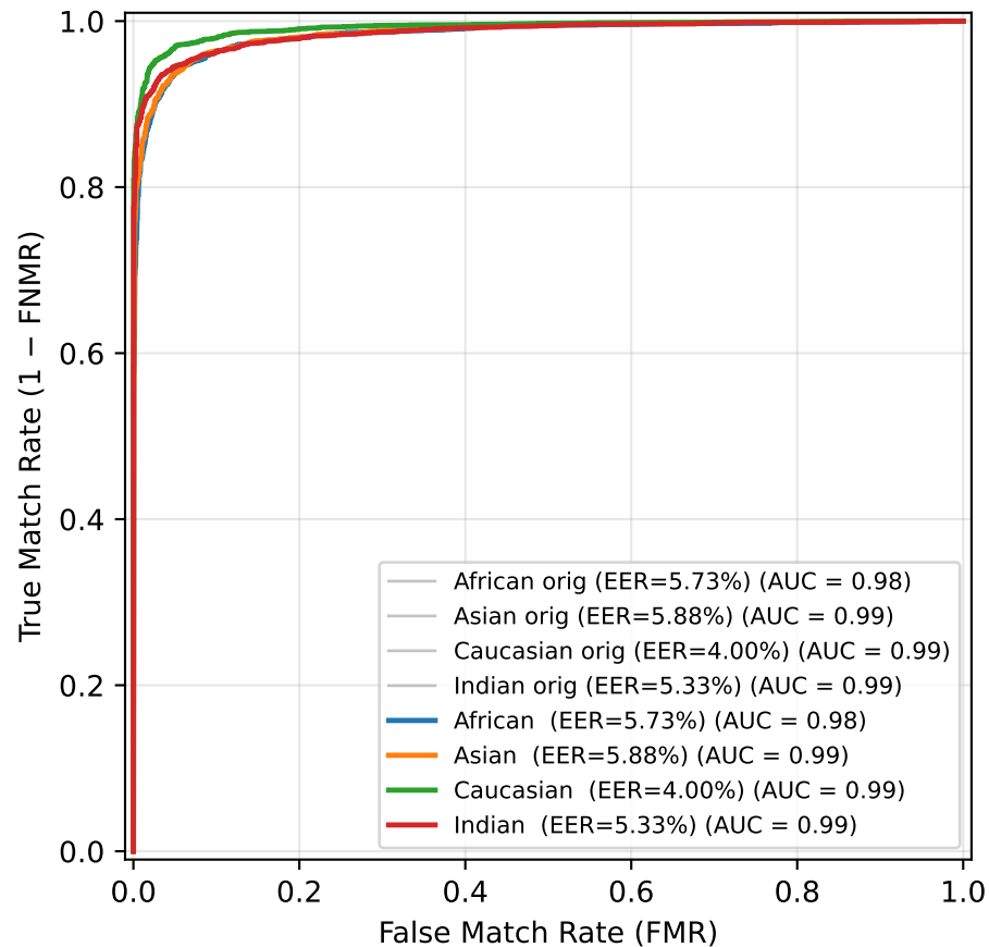
ROC — Gaussian Blur ( \sigma=0.2 )
