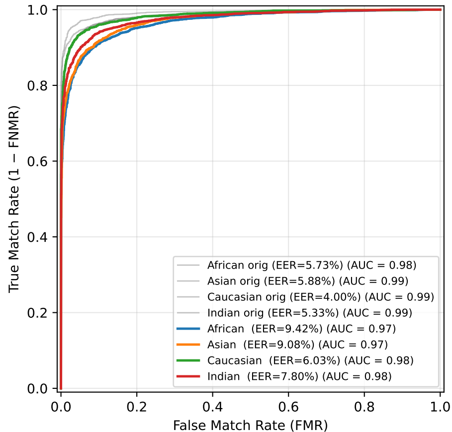
ROC — Gaussian Blur ( \sigma=1.4 )
