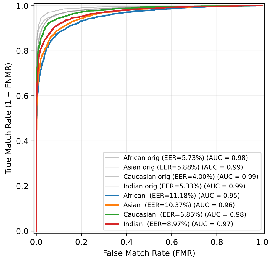
ROC — Gaussian Blur ( \sigma=1.6 )
