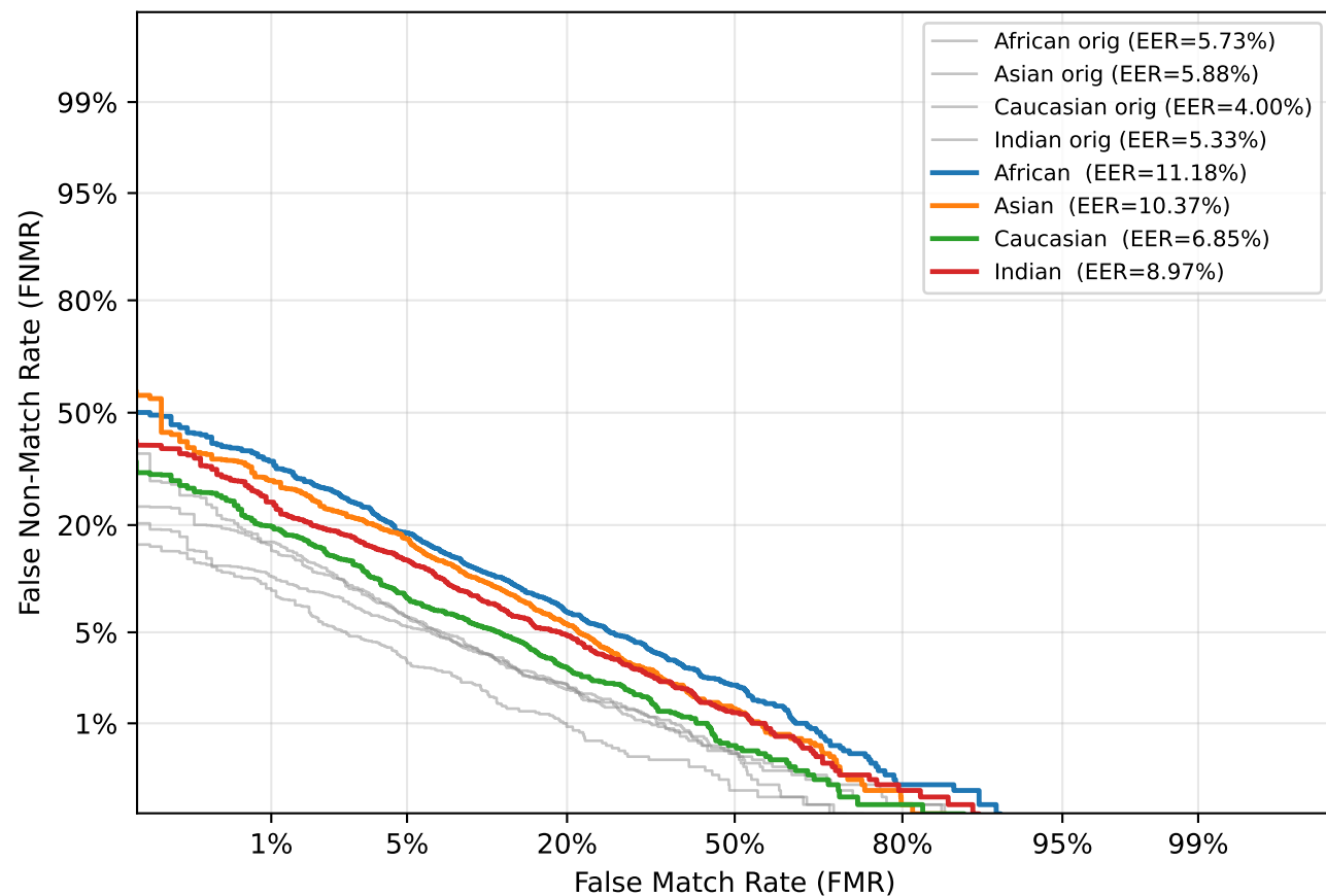
DET — Gaussian Blur ( \sigma=1.6 )
