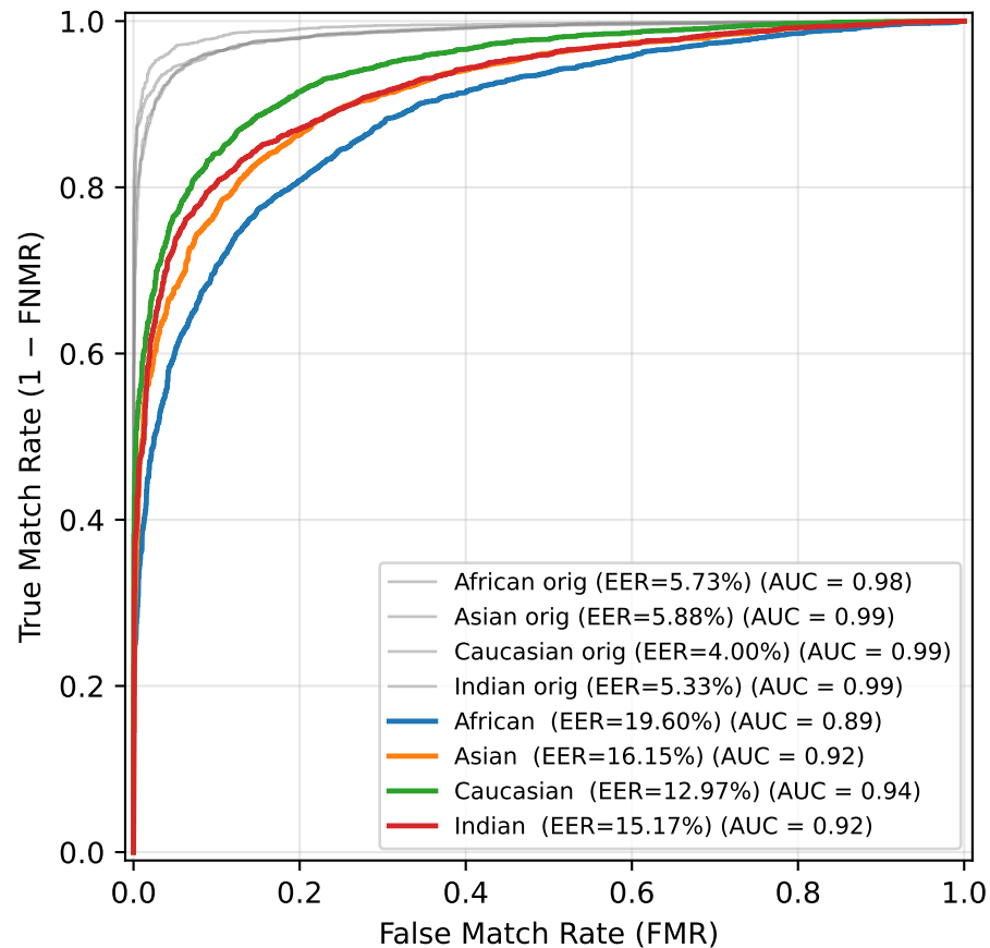
ROC — Gaussian Blur ( \sigma=2.4 )
