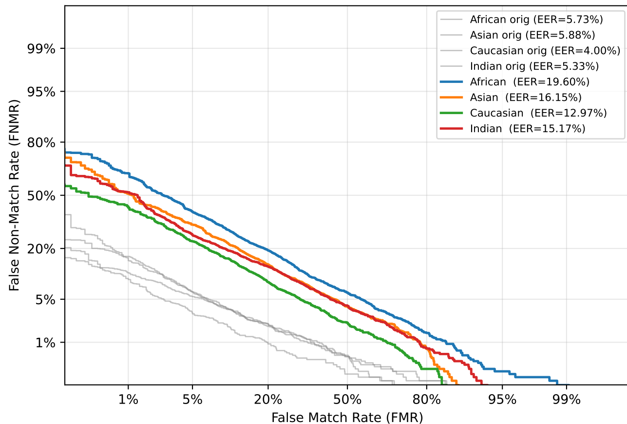
DET — Gaussian Blur ( \sigma=2.4 )
