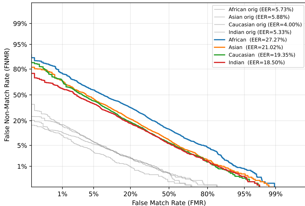
DET — Gaussian Noise ( \sigma=30 )
