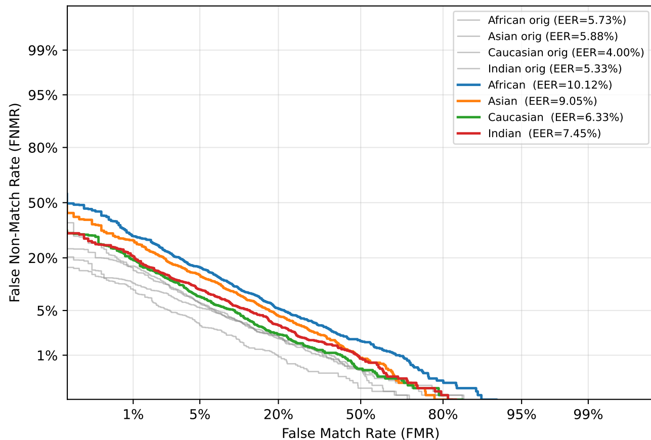
DET — Gaussian Noise ( \sigma=8 )
