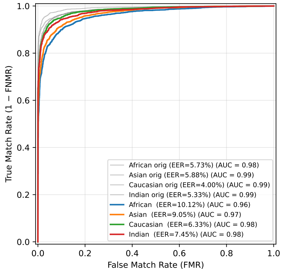
ROC — Gaussian Noise ( \sigma=8 )
