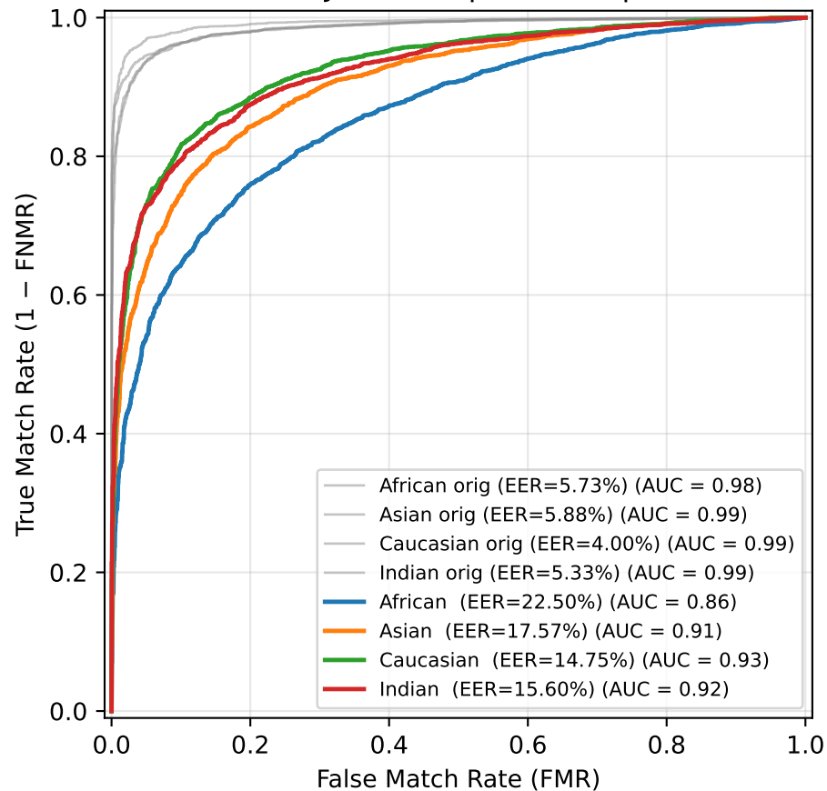
ROC — JPEG Compression (q=10)
