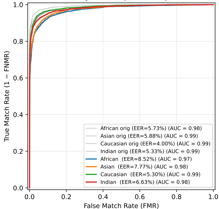
ROC — JPEG Compression (q=40)
