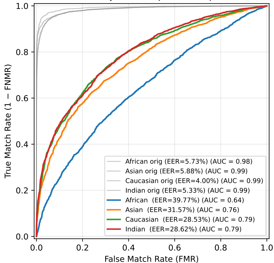
ROC — JPEG Compression (q=5)
