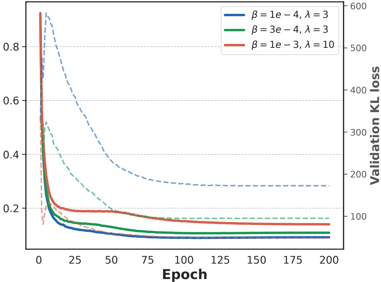
Validation recon loss
