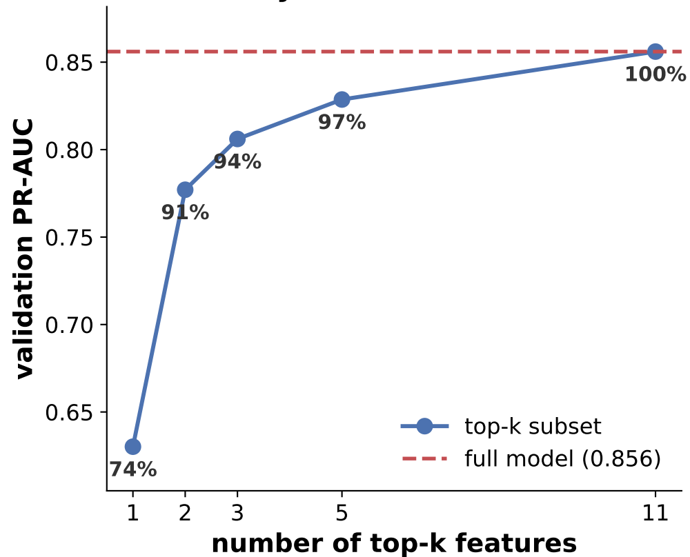
(b) Parsimony: PR-AUC vs feature count
