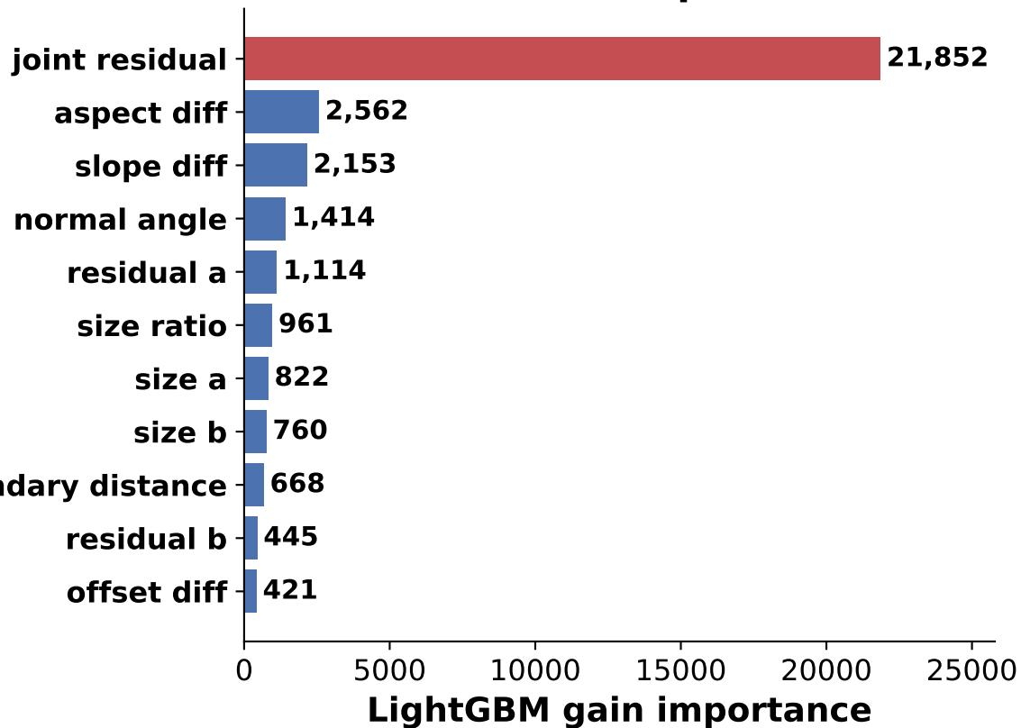
(a) Feature importance
