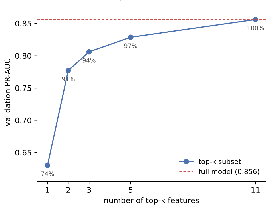
(b) Parsimony: PR-AUC vs feature count
