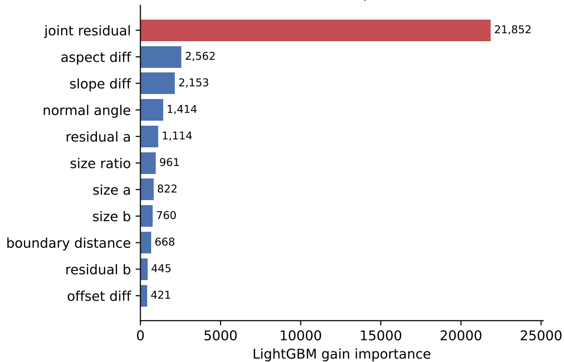
(a) Feature importance
