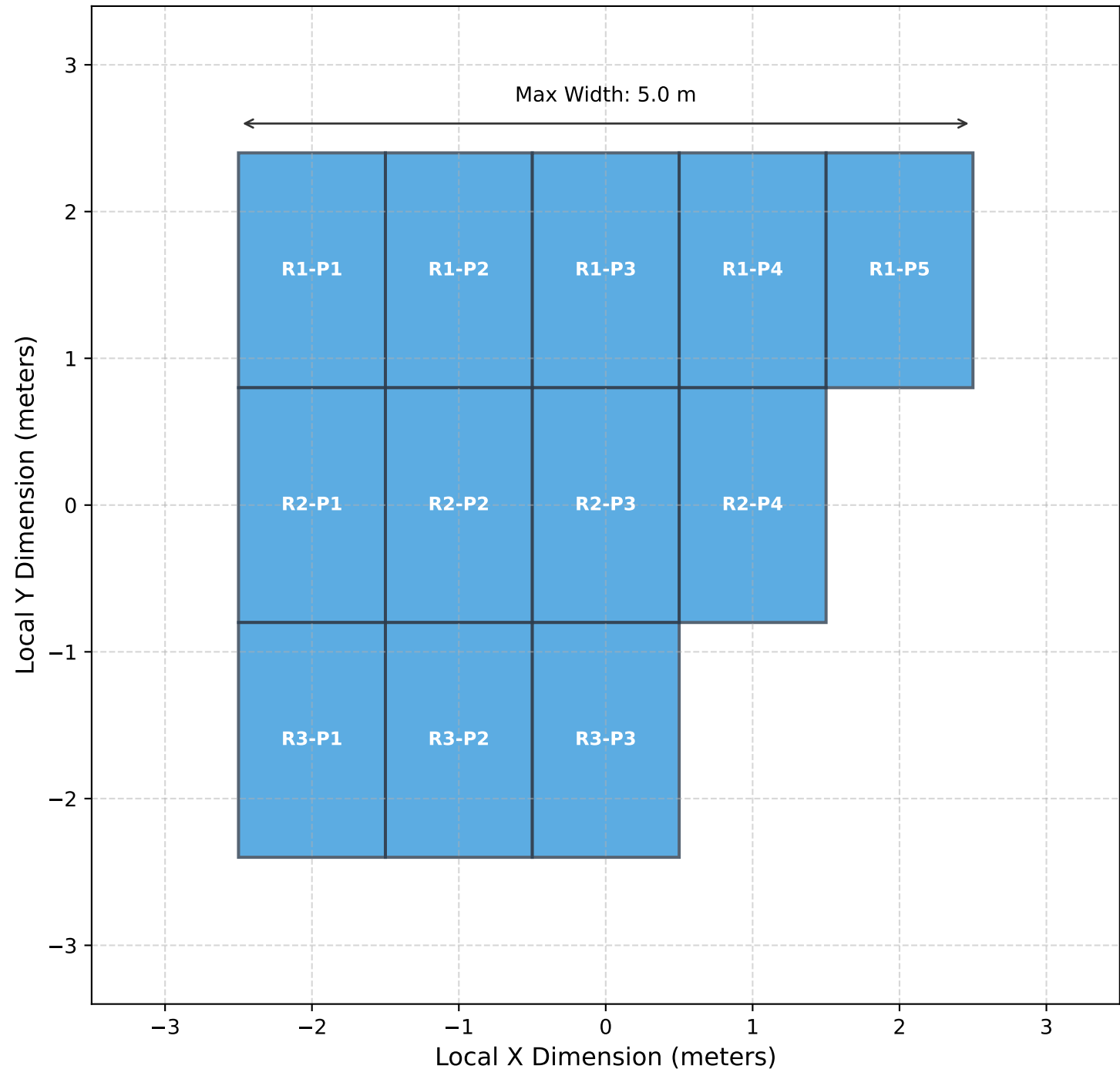
Top-Down Footprint: 5-4-3 PV Array (Left-Aligned) (Azimuth: 170° | Tilt: 12°)
