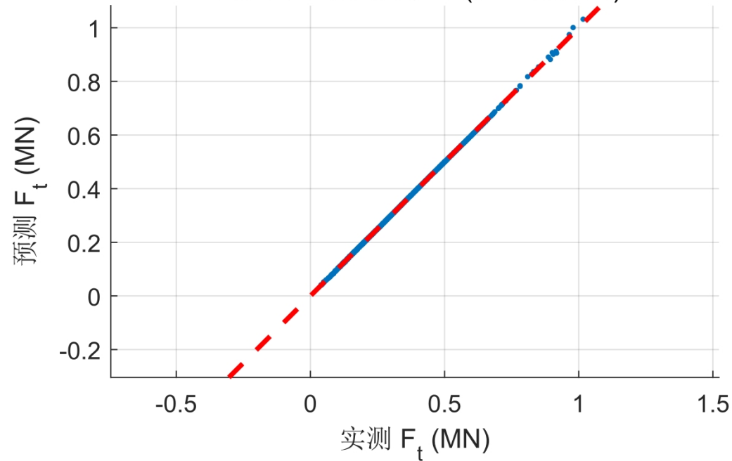
塔架推力-非线性拟合 ( R^2 = 0.9999 )
