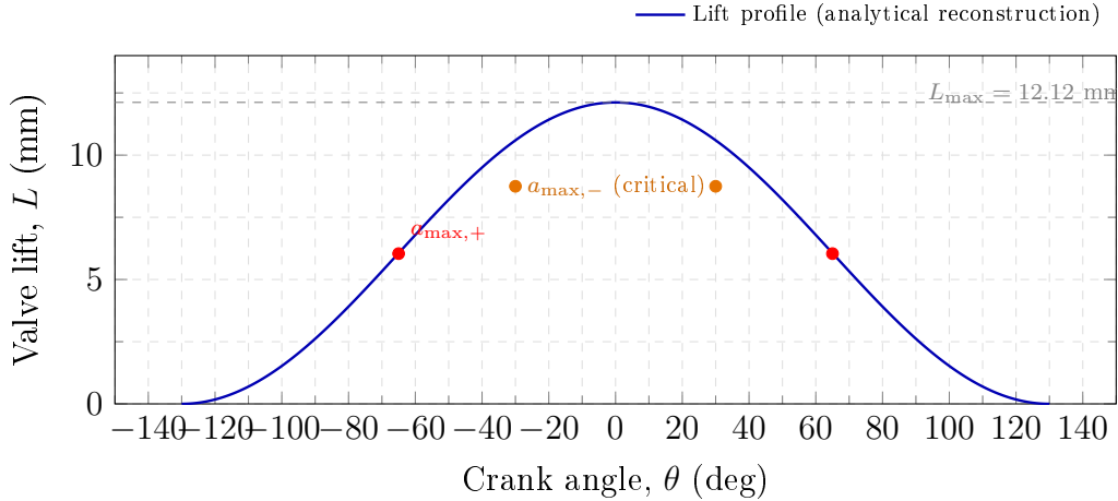
Figure 4: Schematic position of the two critical points of the cam profile of the AP 1.8 high-performance head: positive-acceleration peak ( a_{\text{max},+} = 14\,544 \text{ m s}^{-2} at L_+ = 6.04 \text{ mm} ) and deceleration peak ( a_{\text{max},-} = 20\,362 \text{ m s}^{-2} at L_- = 8.747 \text{ mm} ). The full lift profile is generated from the cam sizing of the intake valve.
