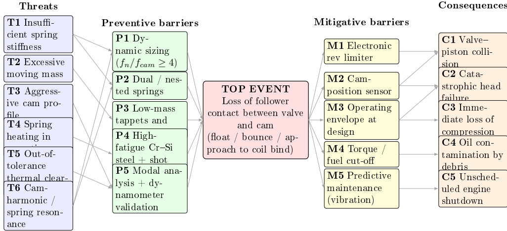
Figure 2: BowTie diagram of the valve train of the AP 1.8 cylinder head operating at 10 000 rpm. Threats (T1–T6) and preventive barriers (P1–P5) are arranged on the left side; consequences (C1–C5) and mitigative barriers (M1–M5) are arranged on the right side. The top event is the loss of follower contact between the valve and the cam, which encompasses valve float, valve bounce, and approach to coil bind.
