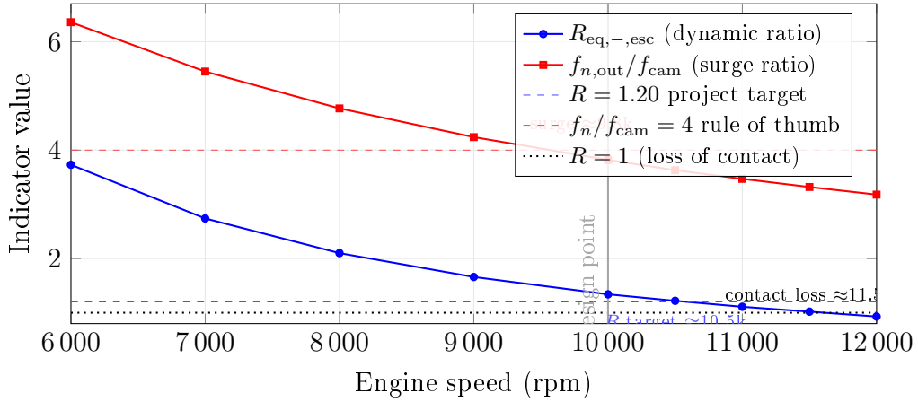
Figure 6: Operating envelope of the AP 1.8 valve train: the dynamic ratio R_{\text{eq},-,\text{esc}} and the outer-spring surge ratio f_{n,\text{out}}/f_{\text{cam}} versus engine speed, from the closed-form scaling of Table 6. The surge rule of thumb is crossed near 9 800 rpm, the dynamic-ratio project target near 10 500 rpm, and the loss-of-contact boundary ( R = 1 ) near 11 500 rpm; the 10 000 rpm design point sits in the most demanding region of the safe envelope.
