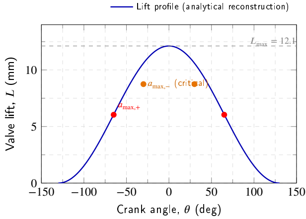
Figure 3: Schematic position of the two critical points of the cam profile of the AP 1.8 high-performance head: positive-acceleration peak ( a_{max,+} = 14\,544\text{ m s}^{-2} at L_+ = 6.04\text{ mm} ) and deceleration peak ( a_{max,-} = 20\,362\text{ m s}^{-2} at L_- = 8.747\text{ mm} ). The full lift profile is generated from the cam sizing of the intake valve.
