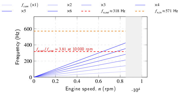
Figure 4: Spring natural frequencies f_{n,out} and f_{n,in} compared with the first six cam harmonics ( n = 1, \dots, 6 ) across the engine-speed range up to 10 000 rpm. The shaded region marks the operating regime; the dashed horizontal lines mark f_{n,out} \approx 318\text{ Hz} and f_{n,in} \approx 571\text{ Hz} .
