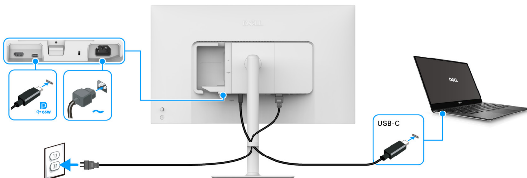
Figure 22. USB-C connection
