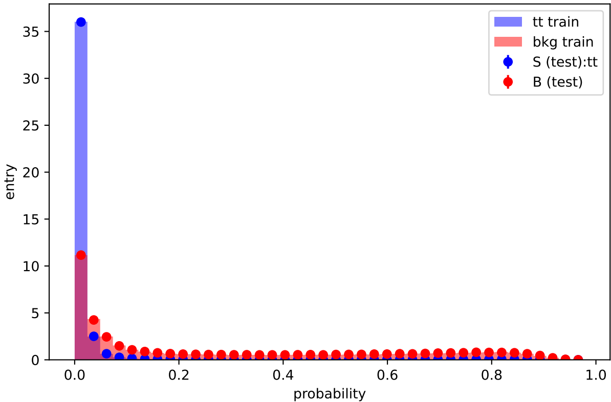
Output distribution
