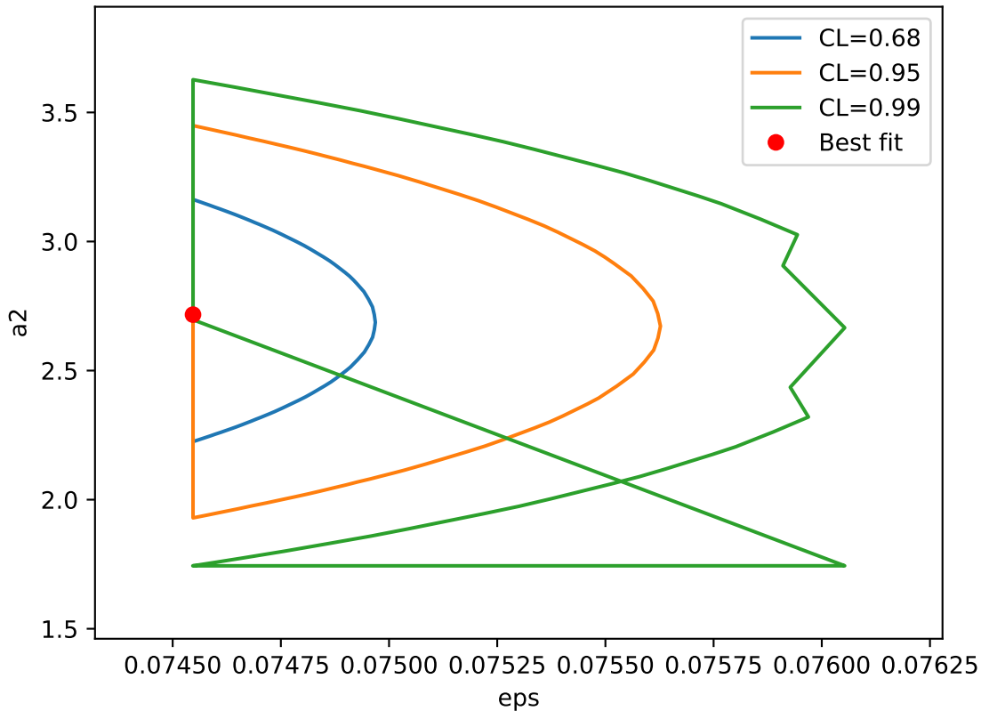
Confidence contours for eps and a2
