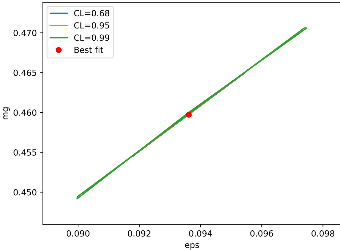
Confidence contours for eps and mg
