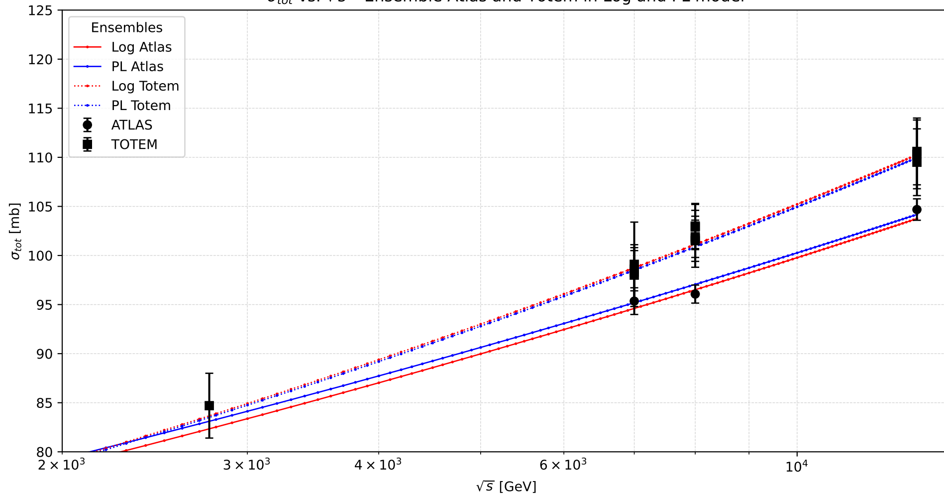
\sigma_{tot} vs. \sqrt{s} - Ensemble Atlas and Totem in Log and PL model
