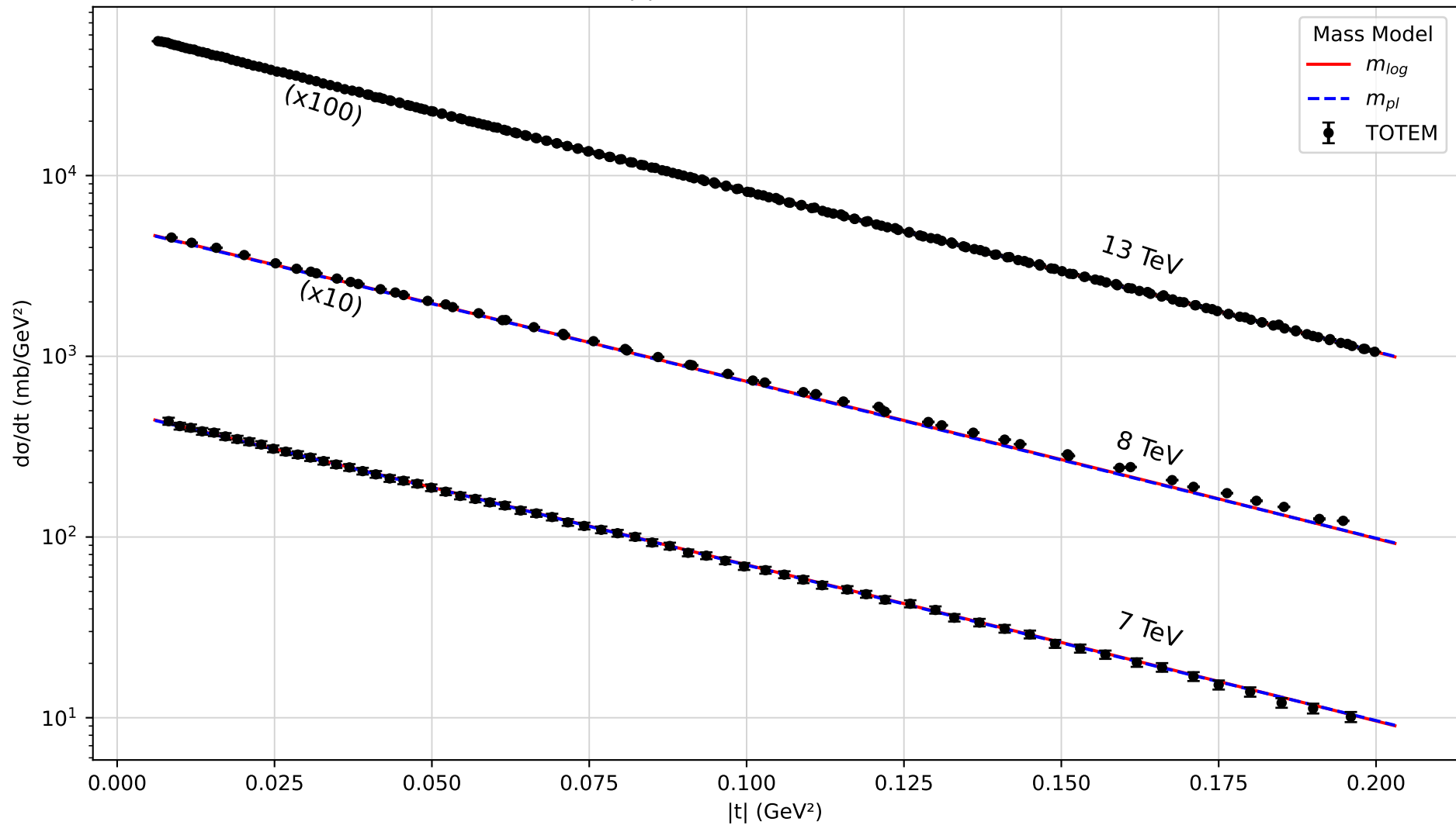
d\sigma/dt vs. |t| - Log and PL models in TOTEM
