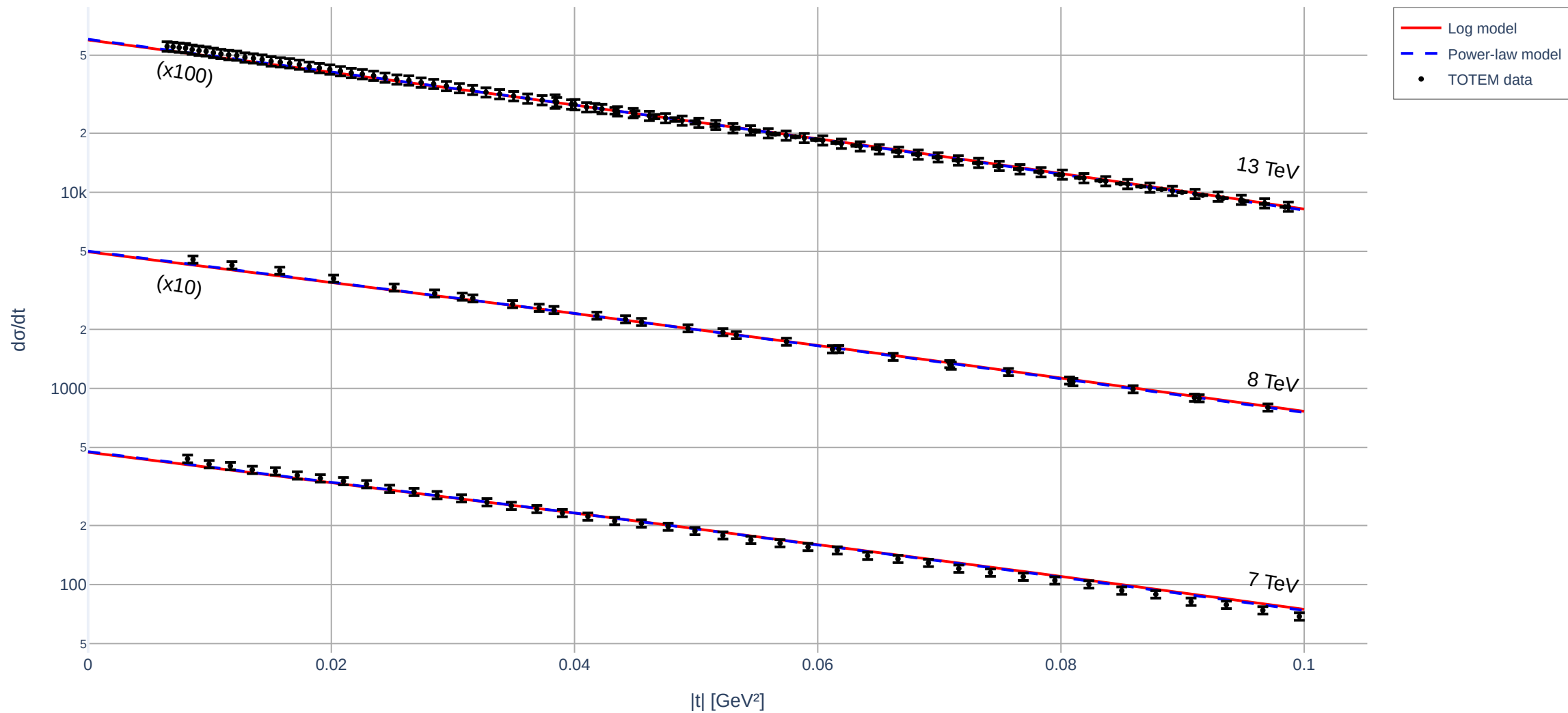
Eikonalized differential cross section (TOTEM Ensemble)
