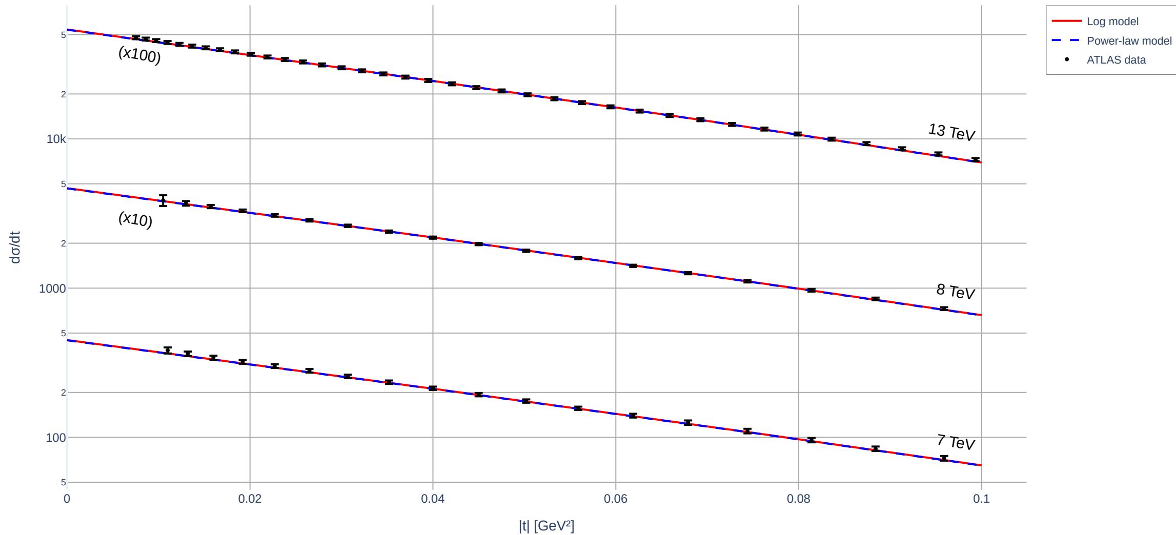
Eikonalized differential cross section (ATLAS Ensemble)
