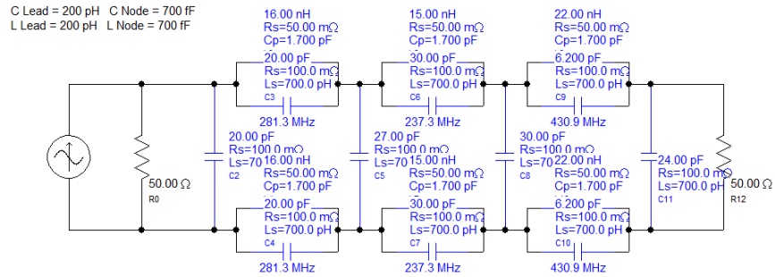
7th Order Low Pass Elliptic Pass Band Frequency = 200.0 MHz Pass Band Ripple = 0.5 dB Stop Band Frequency = 238.0 MHz Stop Band Attenuation = 57.18 dB
