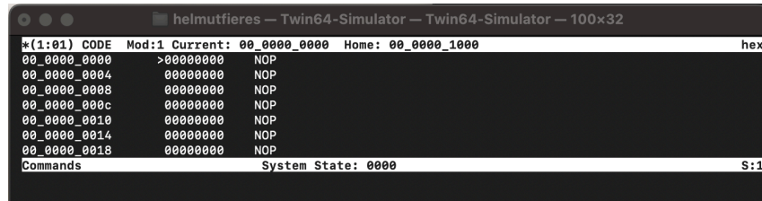
Figure 37: Simulator Memory Window Disassembled Code
