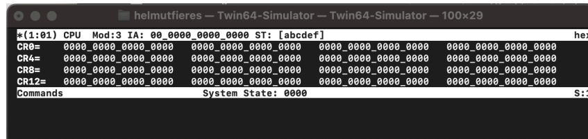
Figure 30: Simulator CPU Window Control Registers
