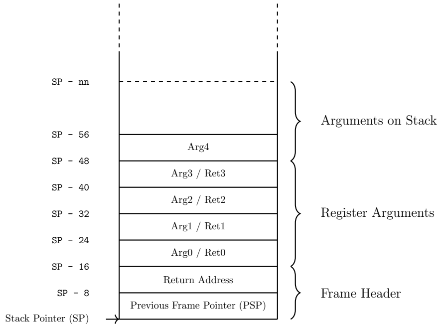
Figure 23: Argument Passing
