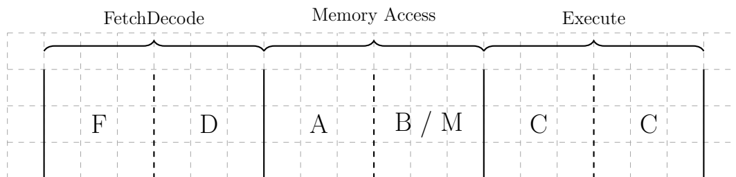
Figure 40: Single Instruction Pipeline
