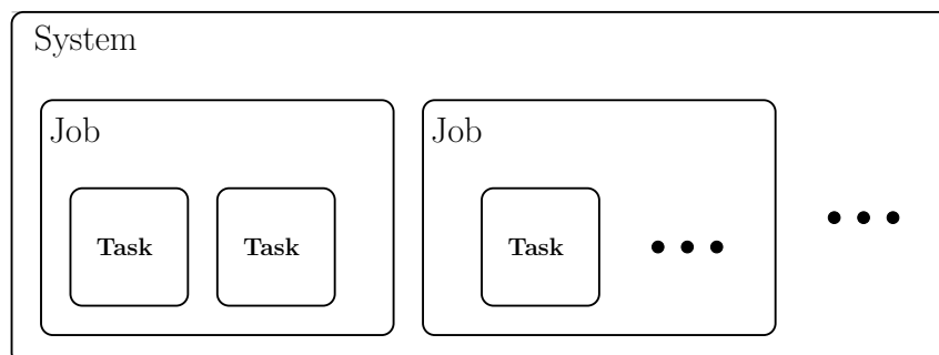
Figure 18: System Environment
