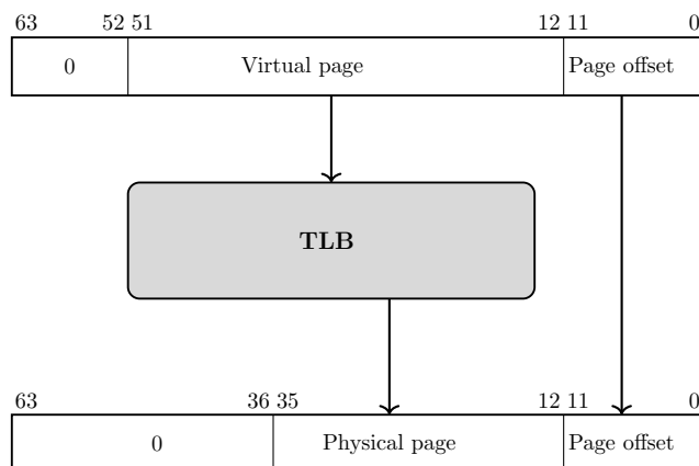
Figure 10: Address translation
