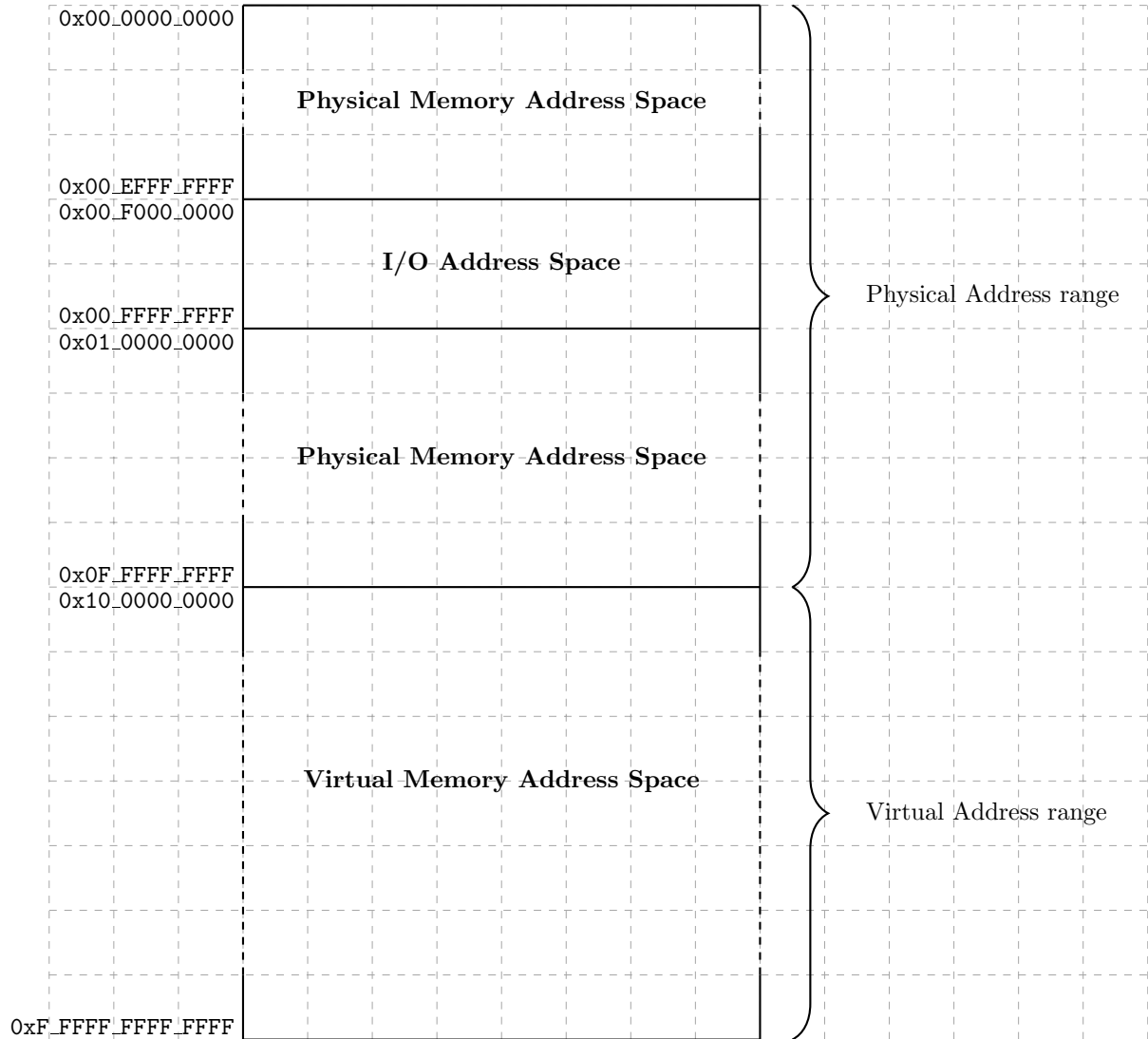
Figure 9: Memory Address Ranges
