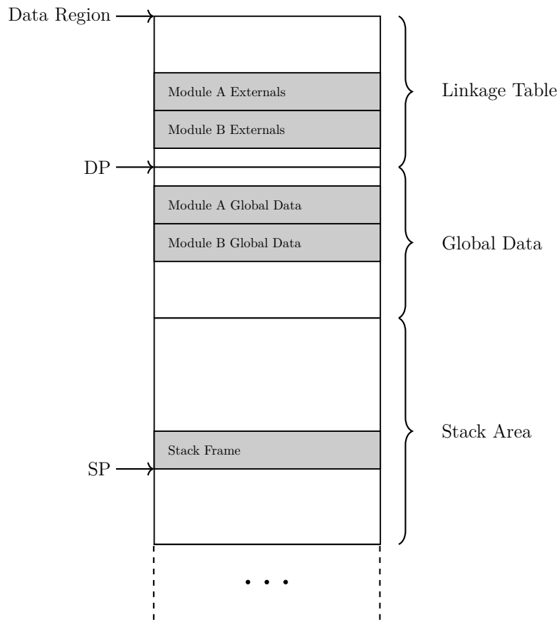
Figure 20: Linkage Table
