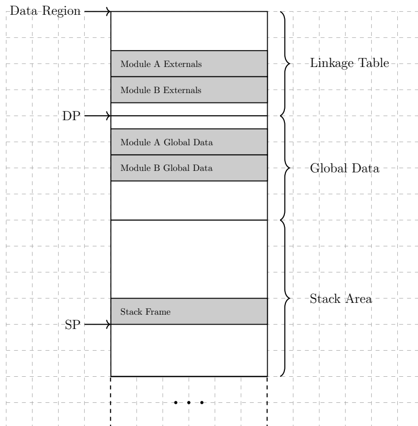
Figure 20: Linkage Table
