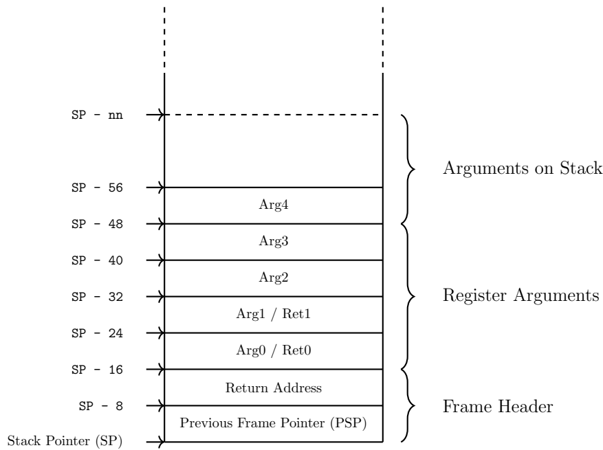
Figure 19: Argument Passing
