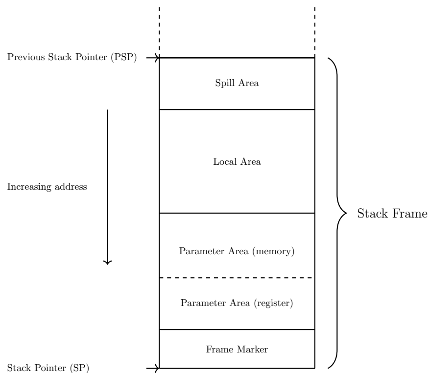
Figure 20: Stack Frame
