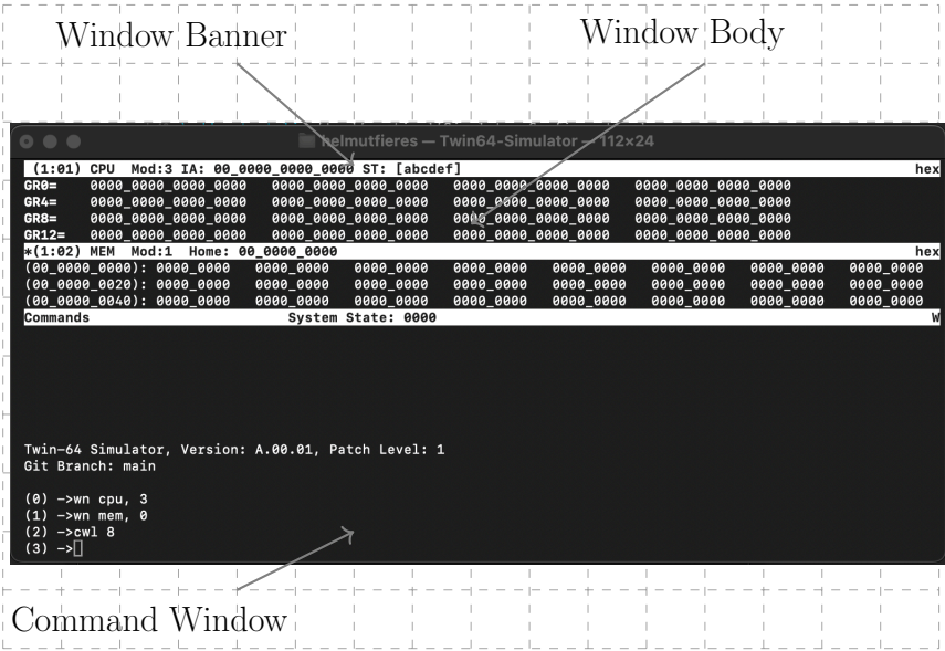
Figure 24: Simulator Environment Screen
