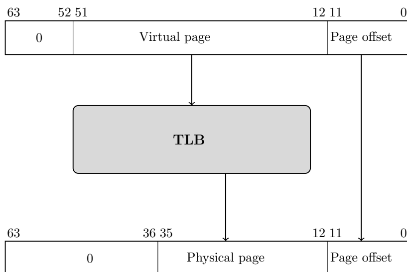
Figure 11: Address translation
