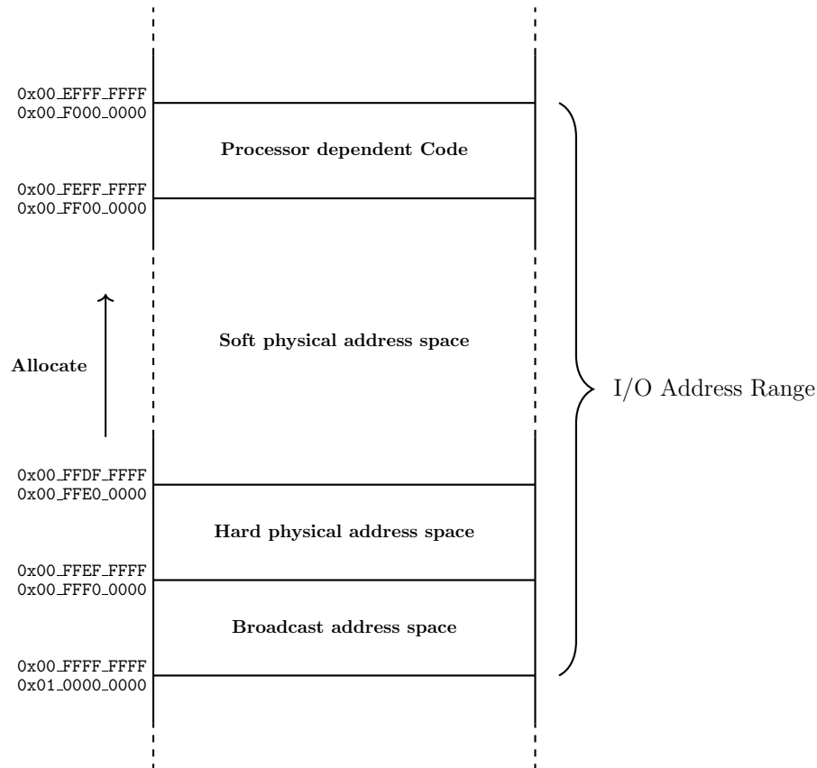
Figure 13: I/O Address Space
