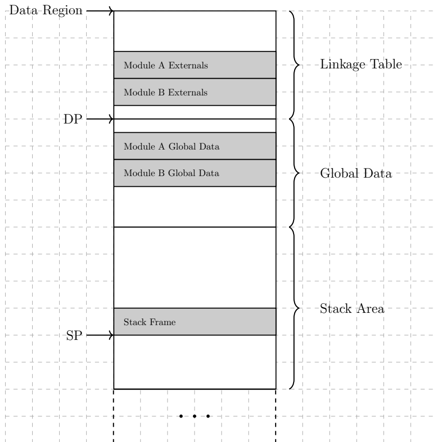
Figure 22: Linkage Table
