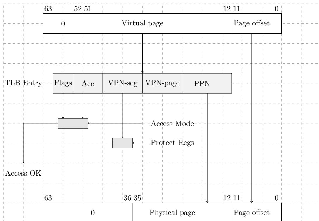
Figure 14: Address translation
