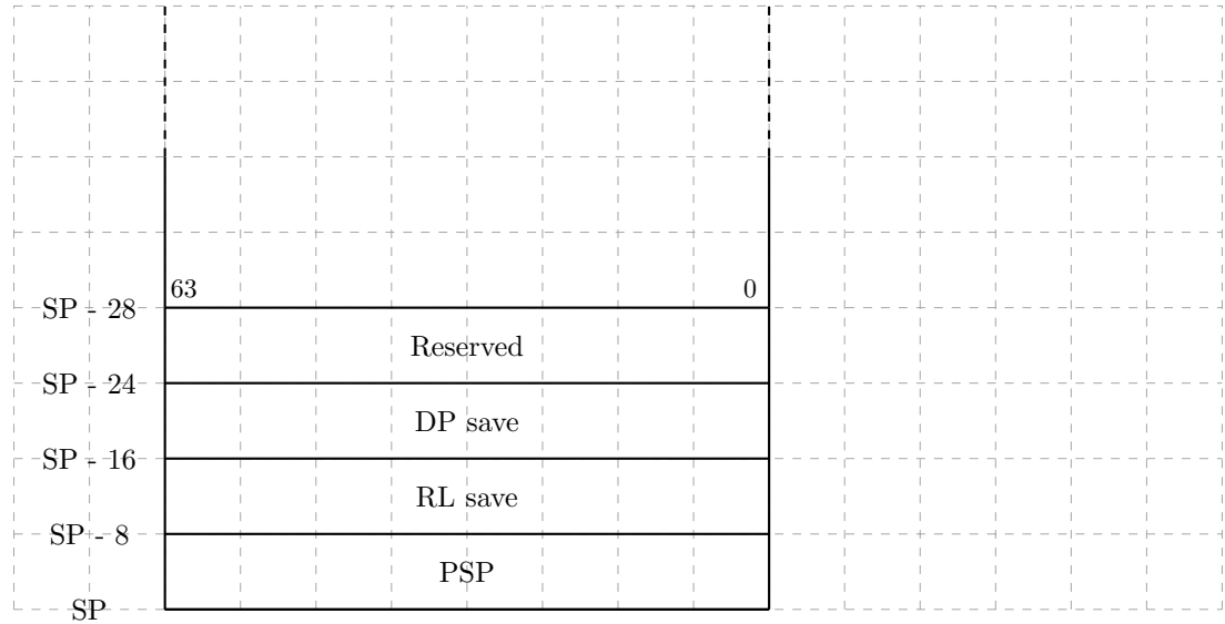
Figure 20: Stack Frame Marker
