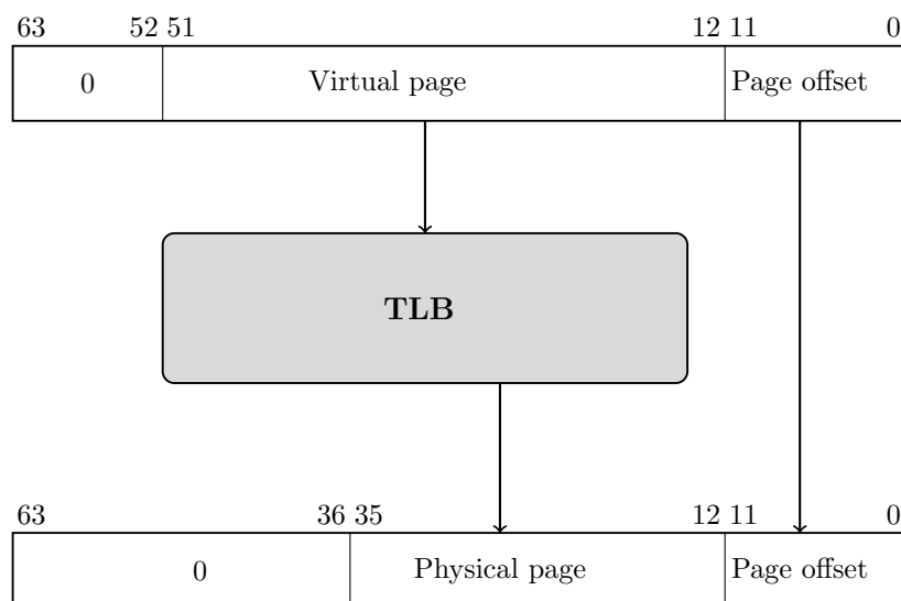
Figure 11: Address translation
