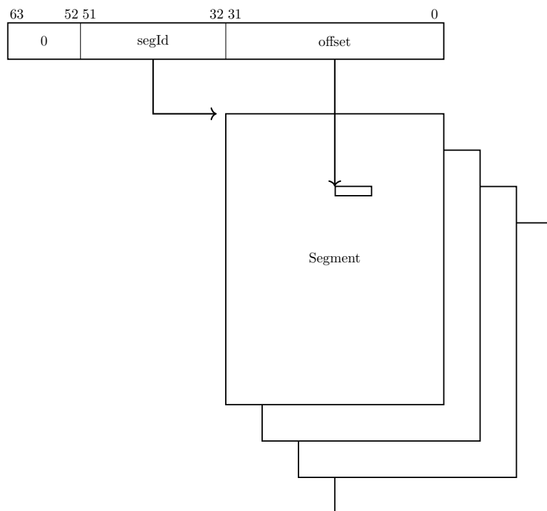
Figure 9: Virtual Memory Address Range
