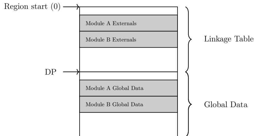
Figure 21: Linkage Table
