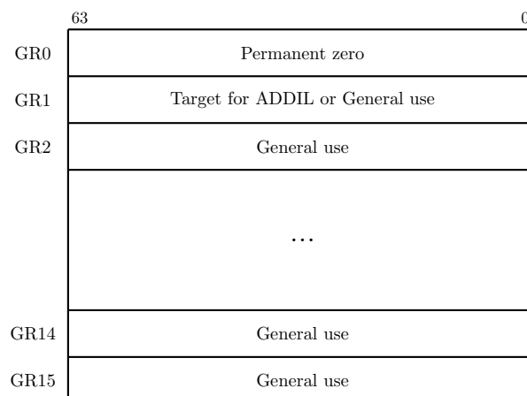
Figure 2: General registers
