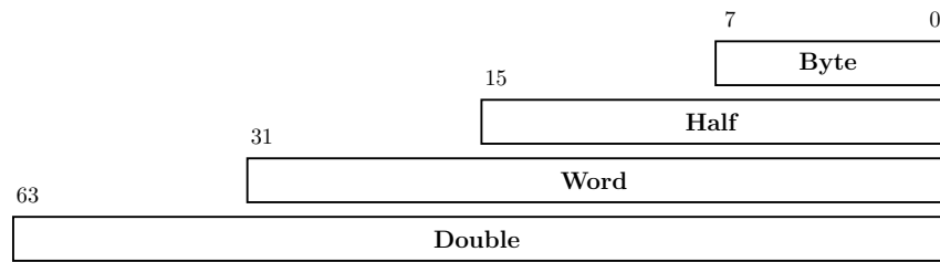
Figure 6: Data types
